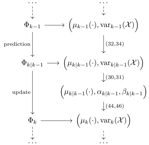
Fig. 1: Data flow of the second-order PHD filter at time k . In addition to the intensity function \mu it propagates the scalar \text{var}(\mathcal{X}) , describing the variance in the estimated number of targets in the whole state space.
