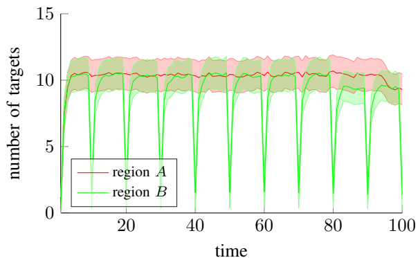
(c) Mean and standard deviation of the estimated target number, PHD filter.
