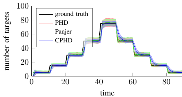
(a) Estimated target number, experiment 2.1.
