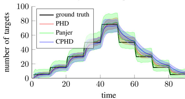
(c) Estimated target number, experiment 2.2.
