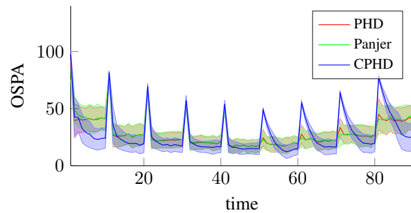
(b) OSPA results, experiment 2.1.
