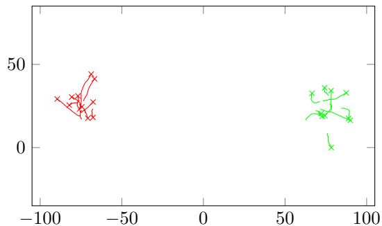
(a) Tracking scenario, with region A on the left and region B on the right.
