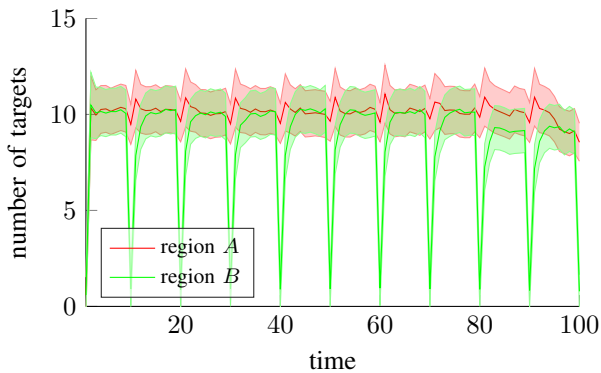
(d) Mean and standard deviation of the estimated target number, Panjer filter.
