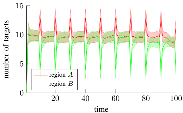
(e) Mean and standard deviation of the estimated target number, CPHD filter.
