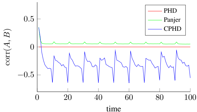
(b) Correlation between the estimated number of targets in regions A and B .
